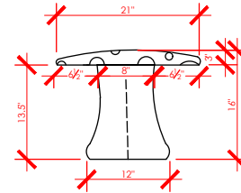
LARGE TOADSTOOL FRONT VIEW DIMENSIONS
