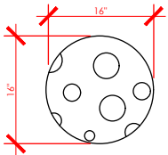
SMALL TOADSTOOL TOP VIEW DIMENSIONS
