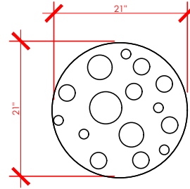
LARGE TOADSTOOL TOP VIEW DIMENSIONS
