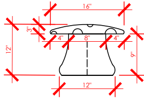
SMALL TOADSTOOL FRONT VIEW DIMENSIONS
